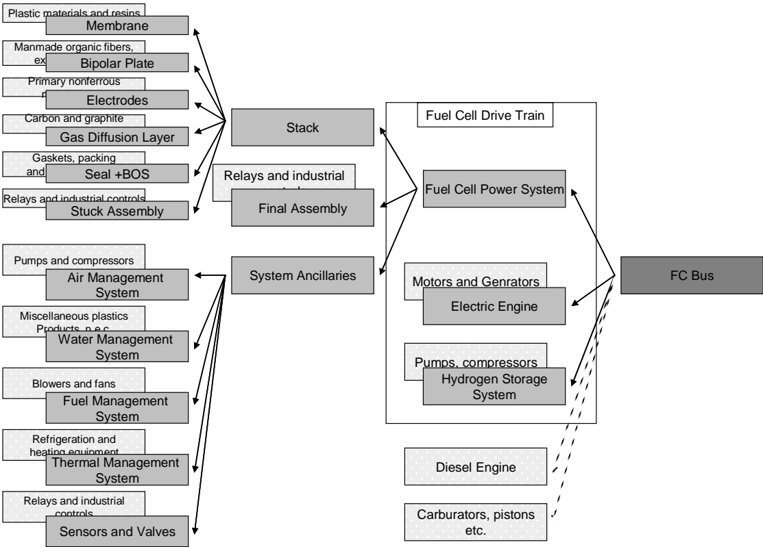
Figure 10: Detailed description of the Fuel Cells Power System by components
