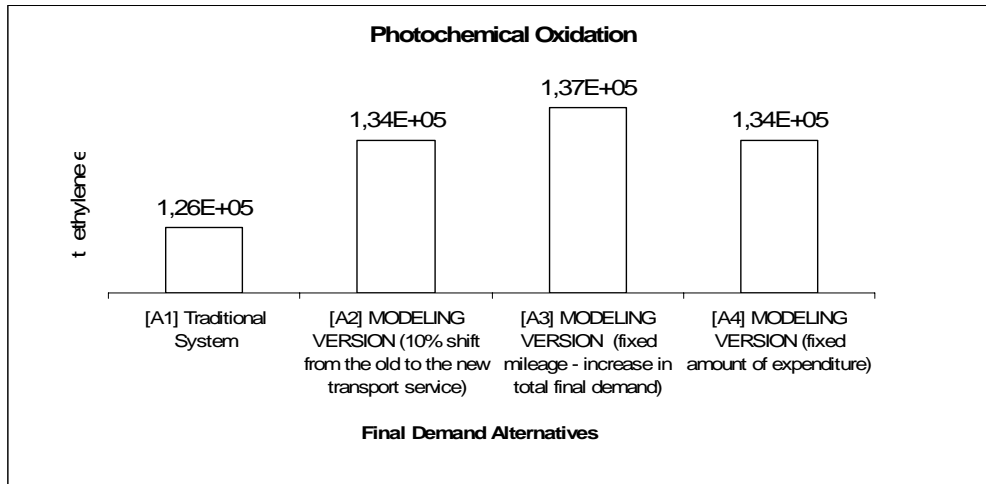
Figure 3: Comparative analysis - Photochemical Oxidation
