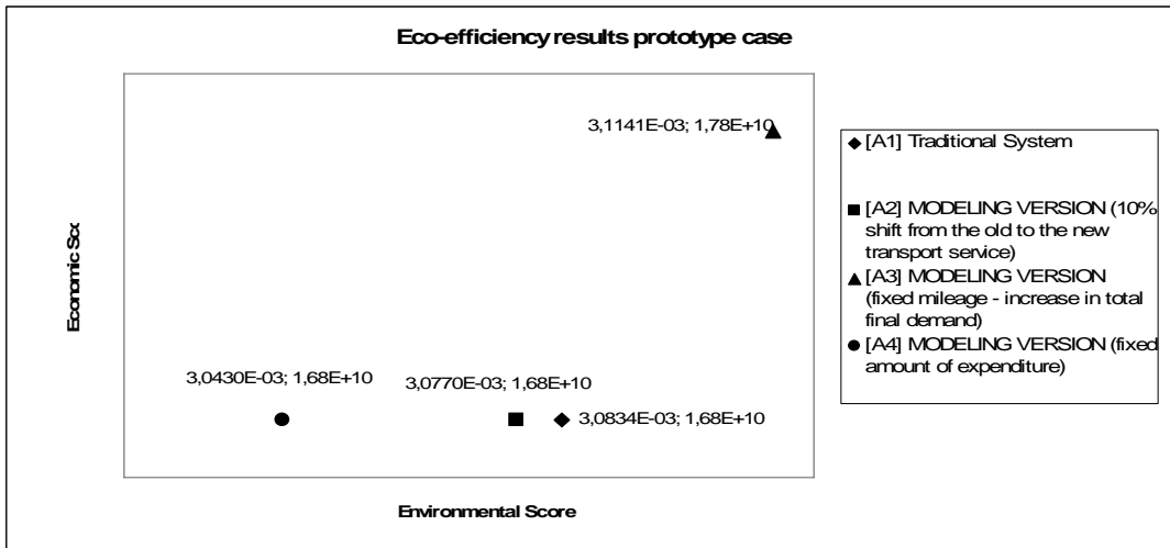
Figure 9: Eco-efficiency results for the prototype case
