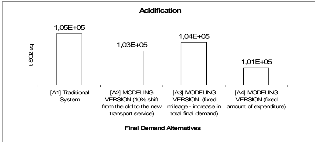
Figure 4: Comparative analysis - Acidification
