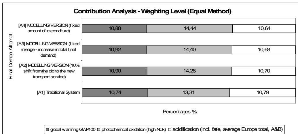
Figure 6: Contribution analysis - weighting level (equal method)
