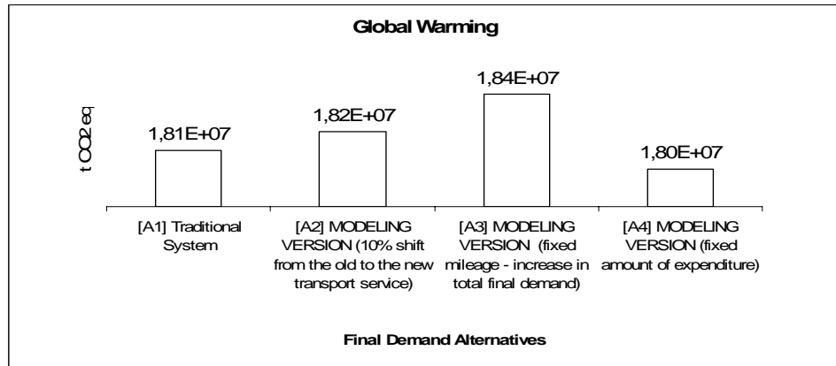
Figure 2: Comparative analysis - Global Warming
