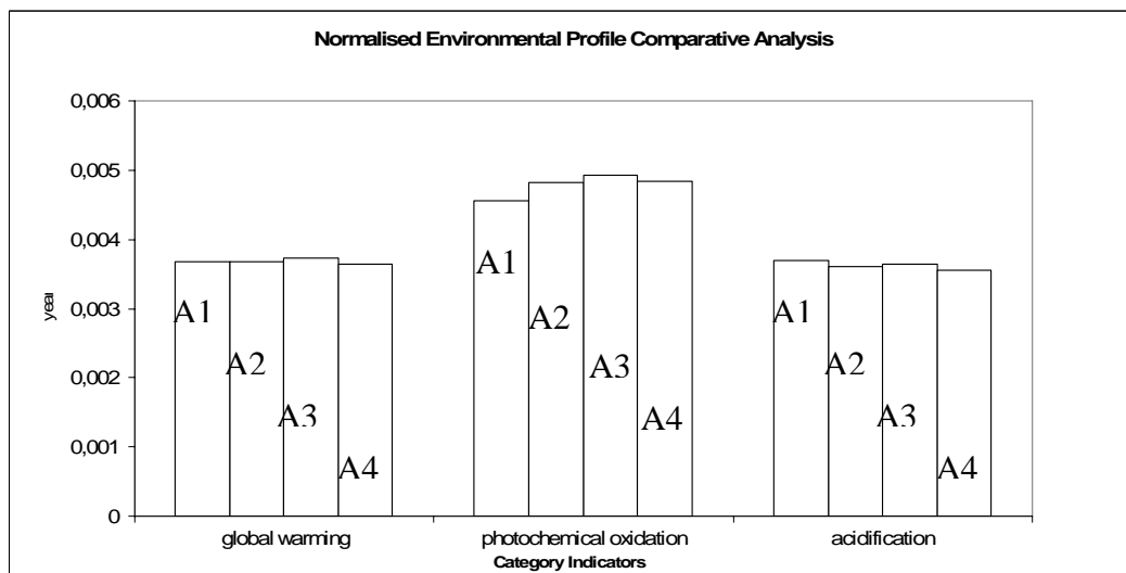
Figure 5: Normalized environmental profile - comparative analysis
