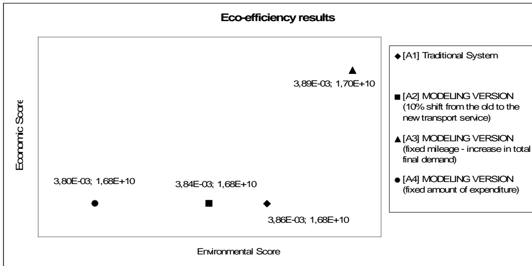
Figure 8: Eco-efficiency results for the mass production case
