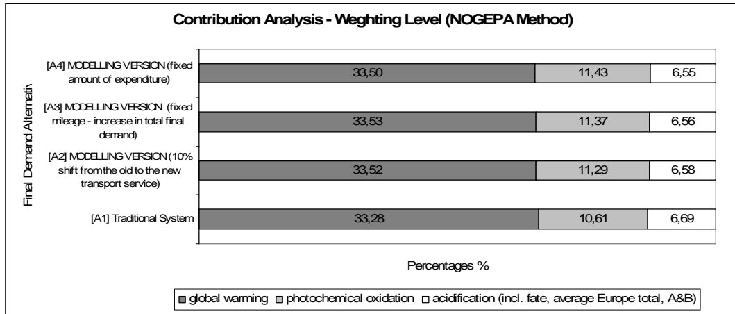
Figure 7: Contribution analysis - weighting level (NOGEPa method)
